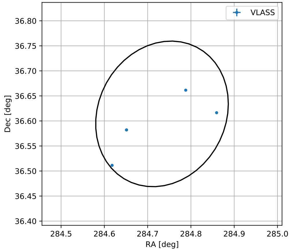
4FGL J1858.9+3636
