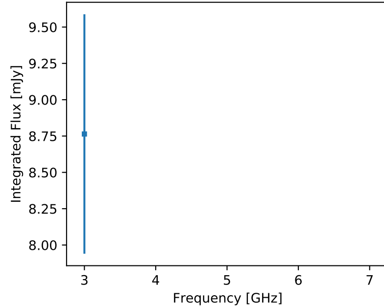
F357 J185821.99-105656.2 (unr)
