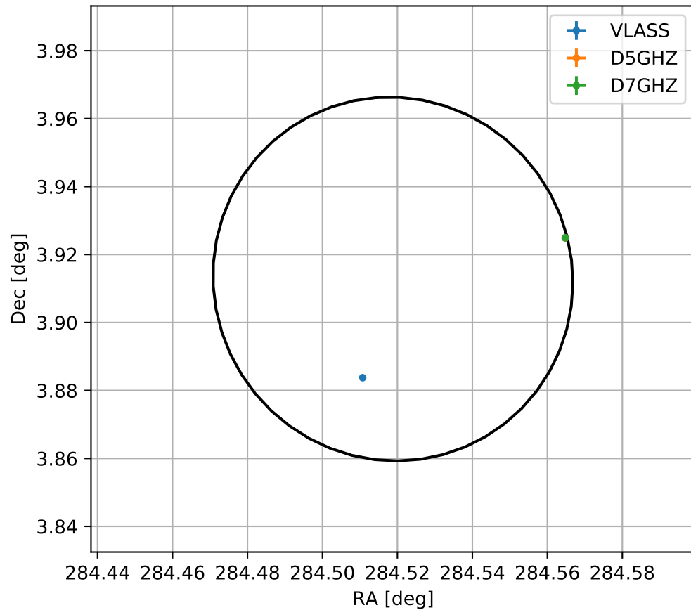
4FGL J1858.0+0354
