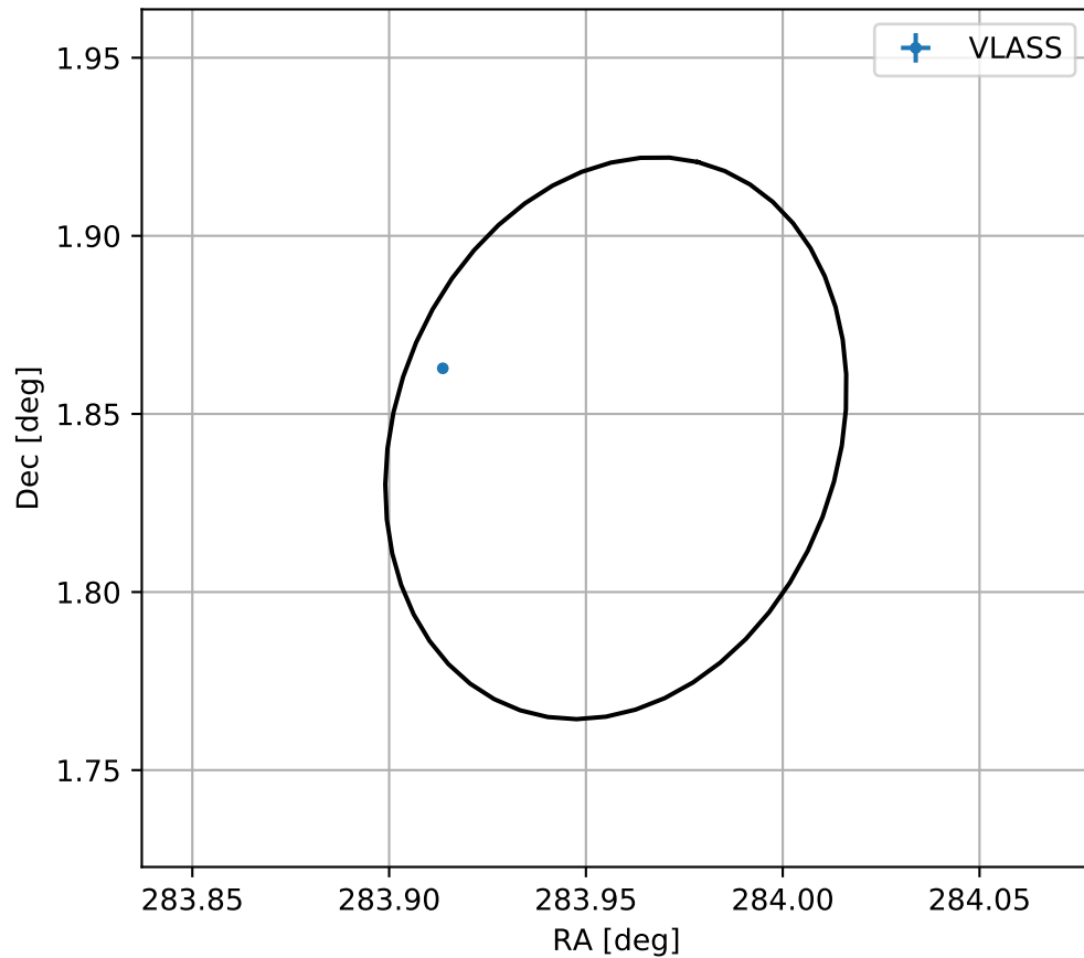
4FGL J1855.8+0150
