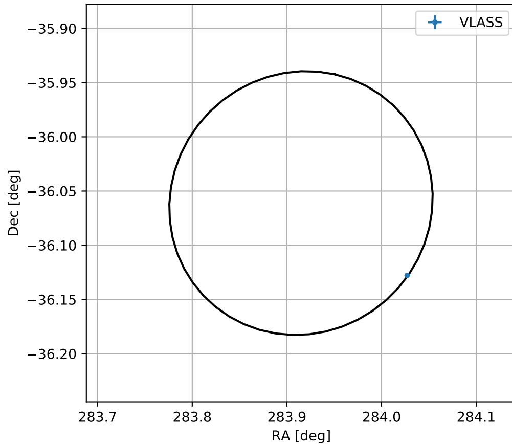
4FGL J1855.6-3603
