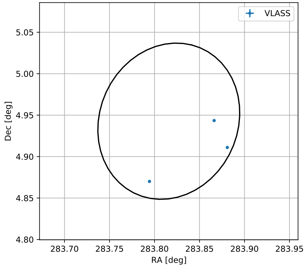
4FGL J1855.2+0456
