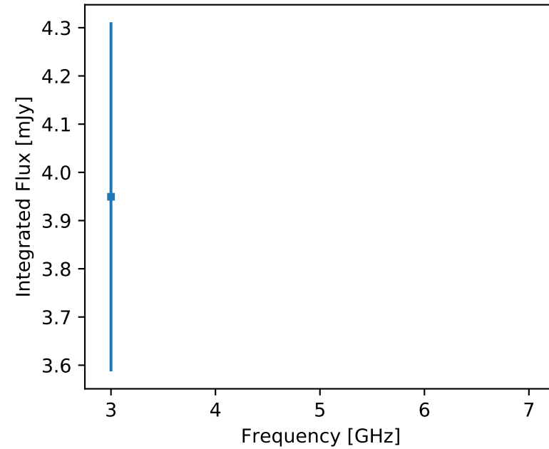
F357 J185441.32+015802.1 (unr)
