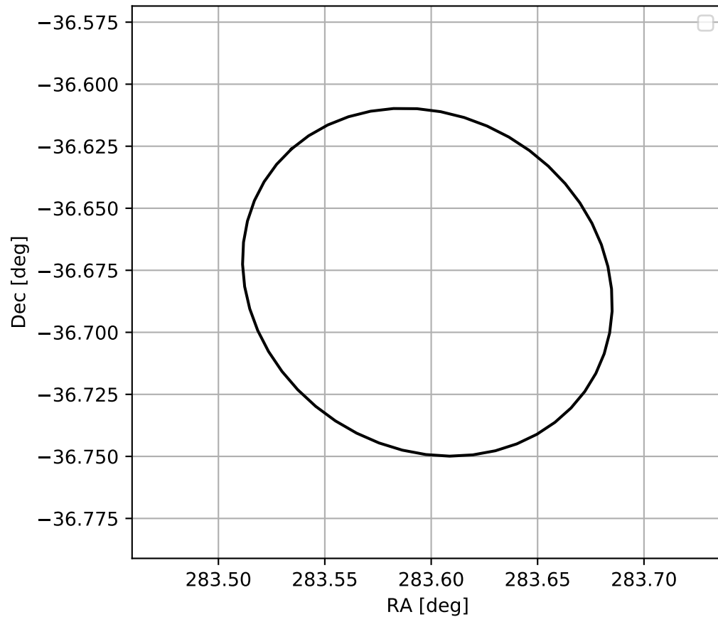
4FGL J1854.3-3640
