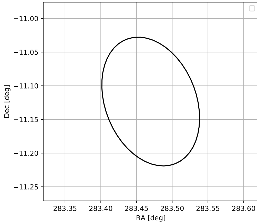
4FGL J1853.8-1107
