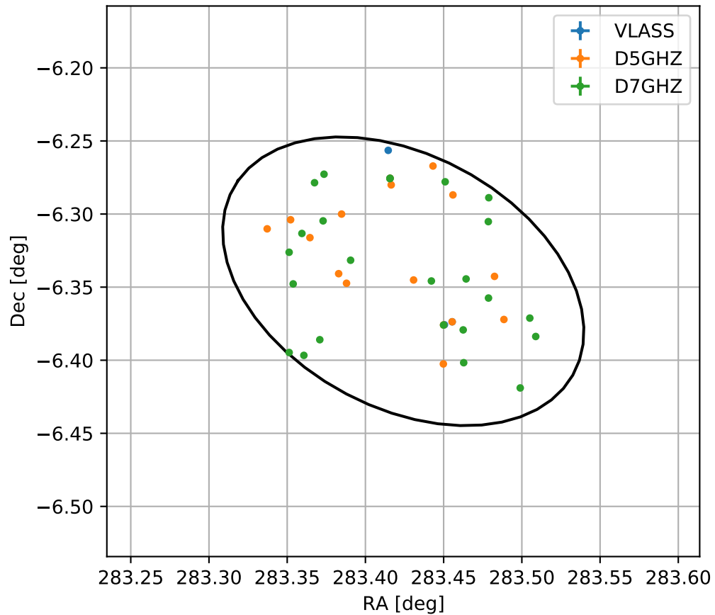
4FGL J1853.6-0620
