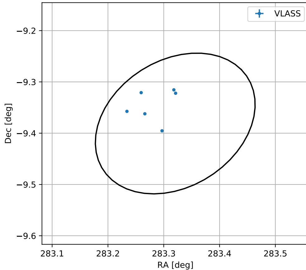
4FGL J1853.2-0922c
