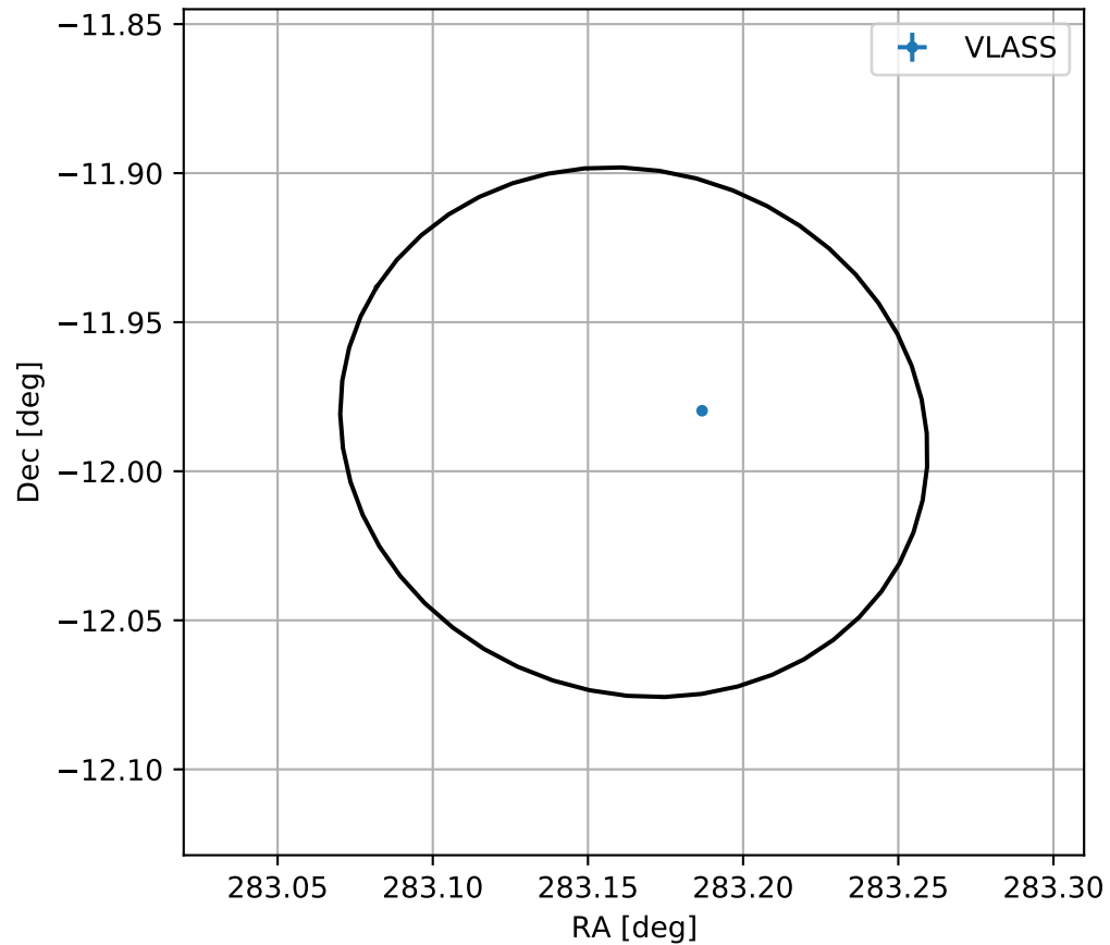
4FGL J1852.6-1159
