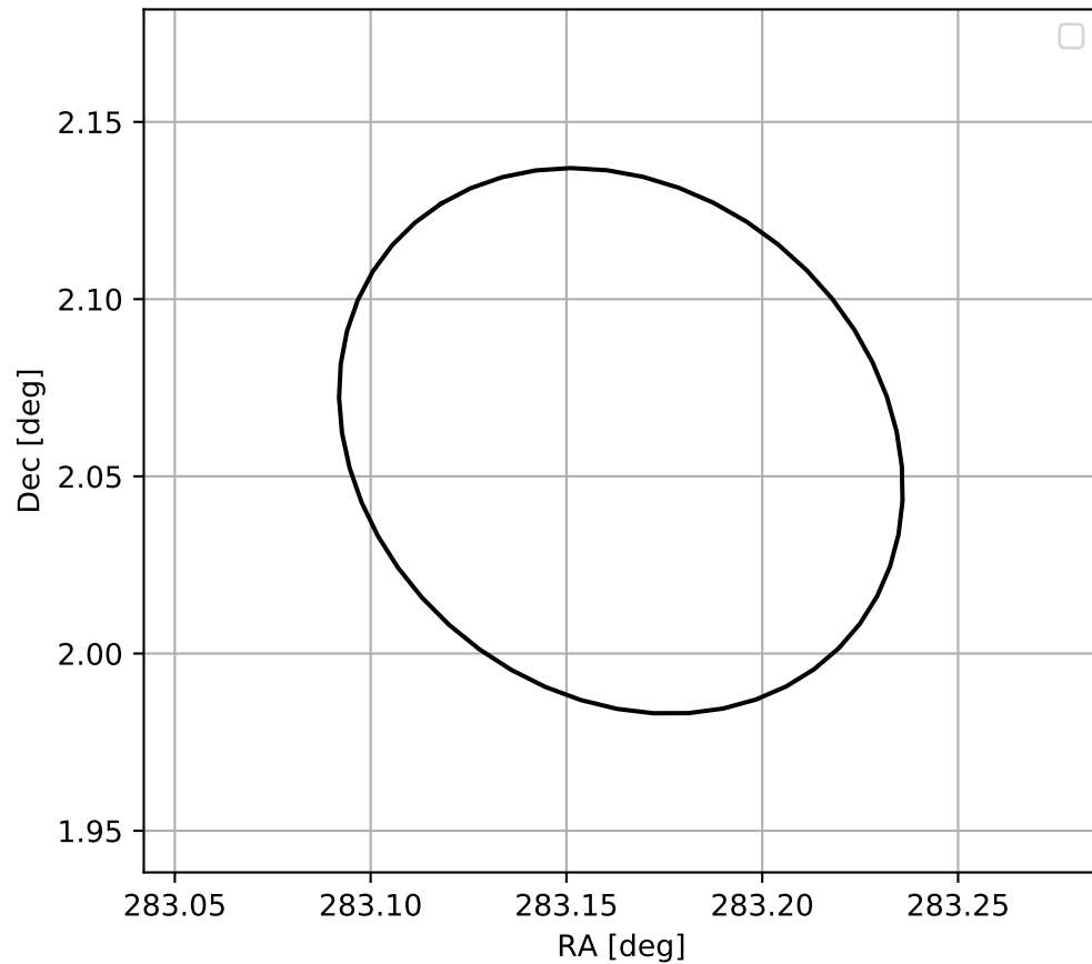
4FGL J1852.6+0203
