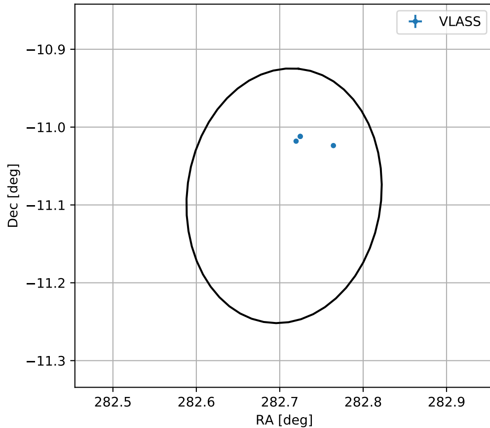
4FGL J1850.8-1105
