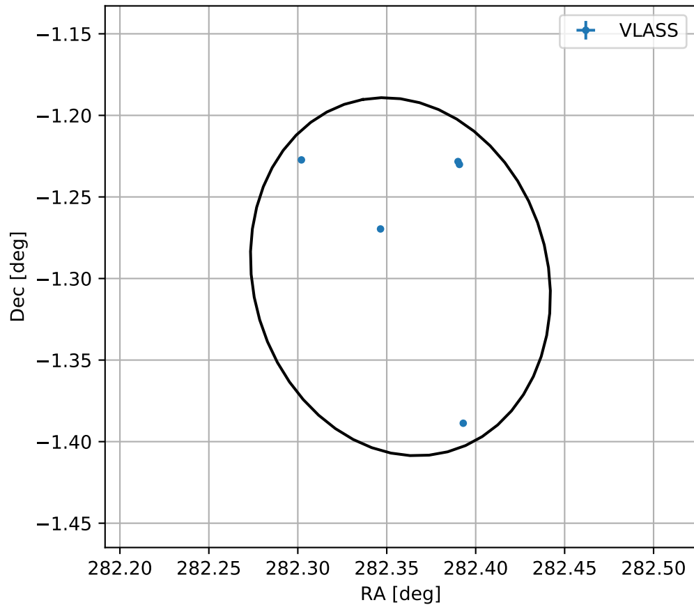
4FGL J1849.4-0117
