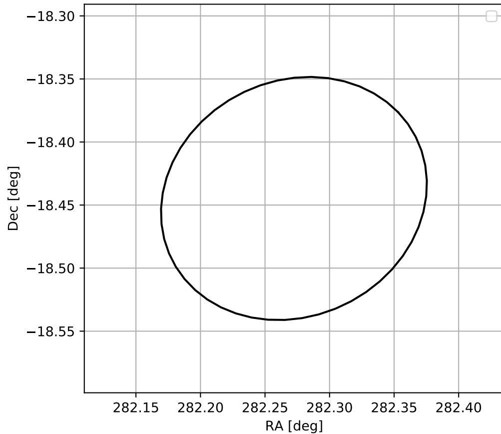
4FGL J1849.0-1826
