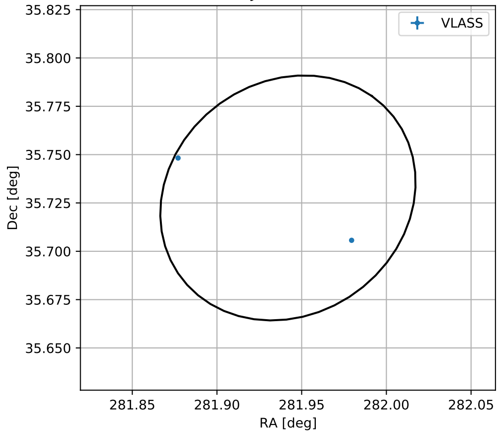
4FGL J1847.7+3543
