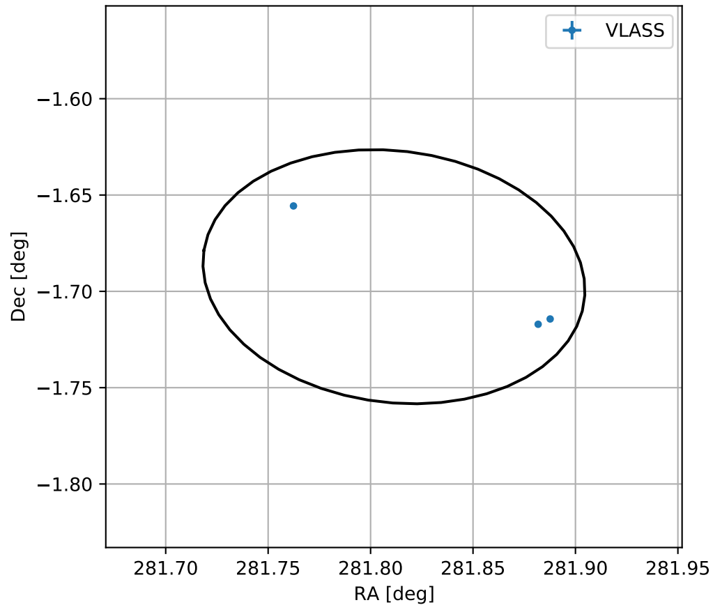
4FGL J1847.2-0141
