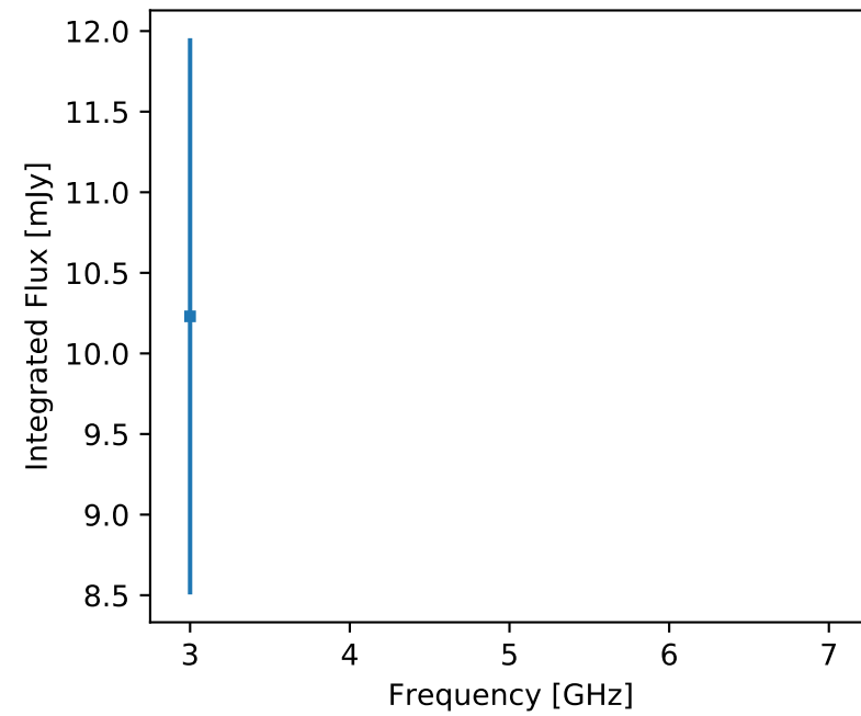
F357 J184733.03-014251.6 (unr)
