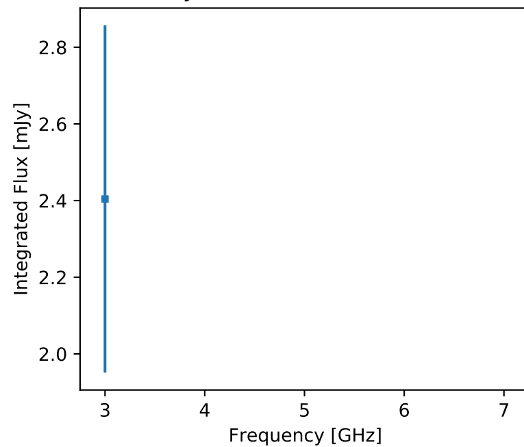
F357 J184731.62-014301.5 (unr)
