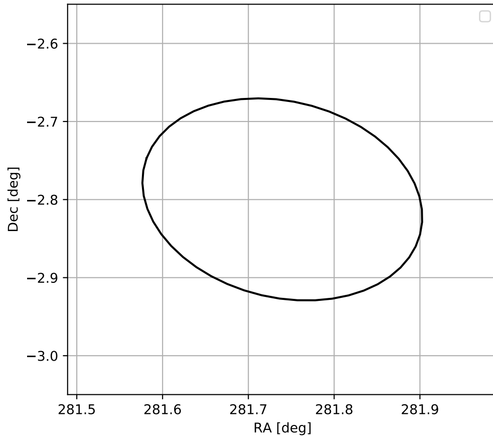
4FGL J1846.9-0247c
