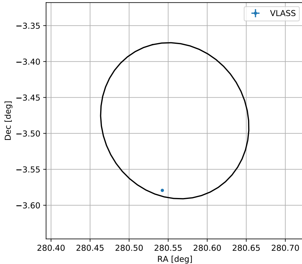
4FGL J1842.2-0328
