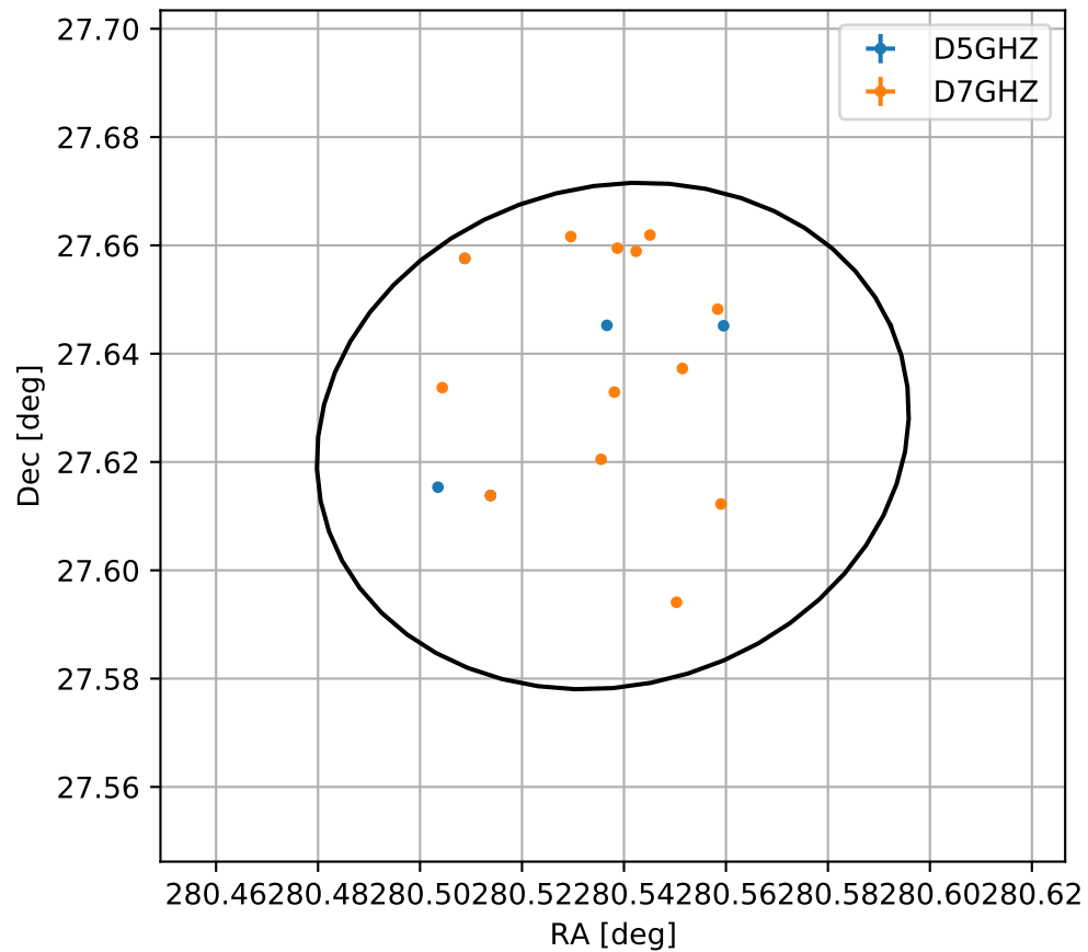
4FGL J1842.1+2737
