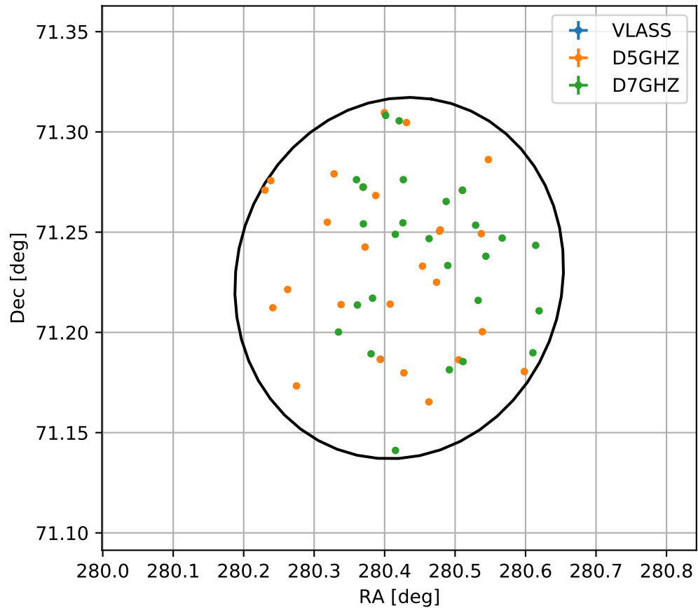
4FGL J1841.6+7113
