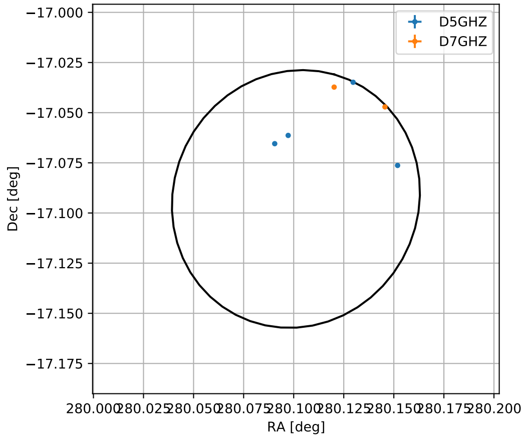
4FGL J1840.4-1705
