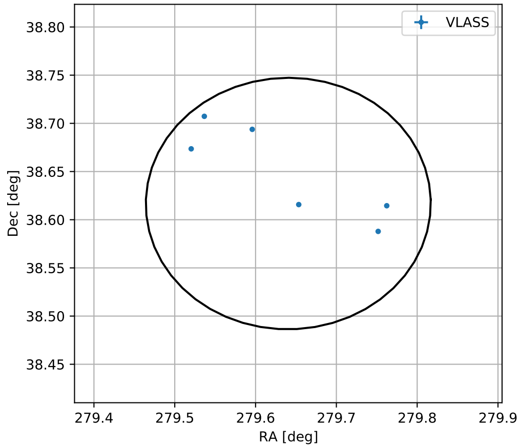
4FGL J1838.5+3837
