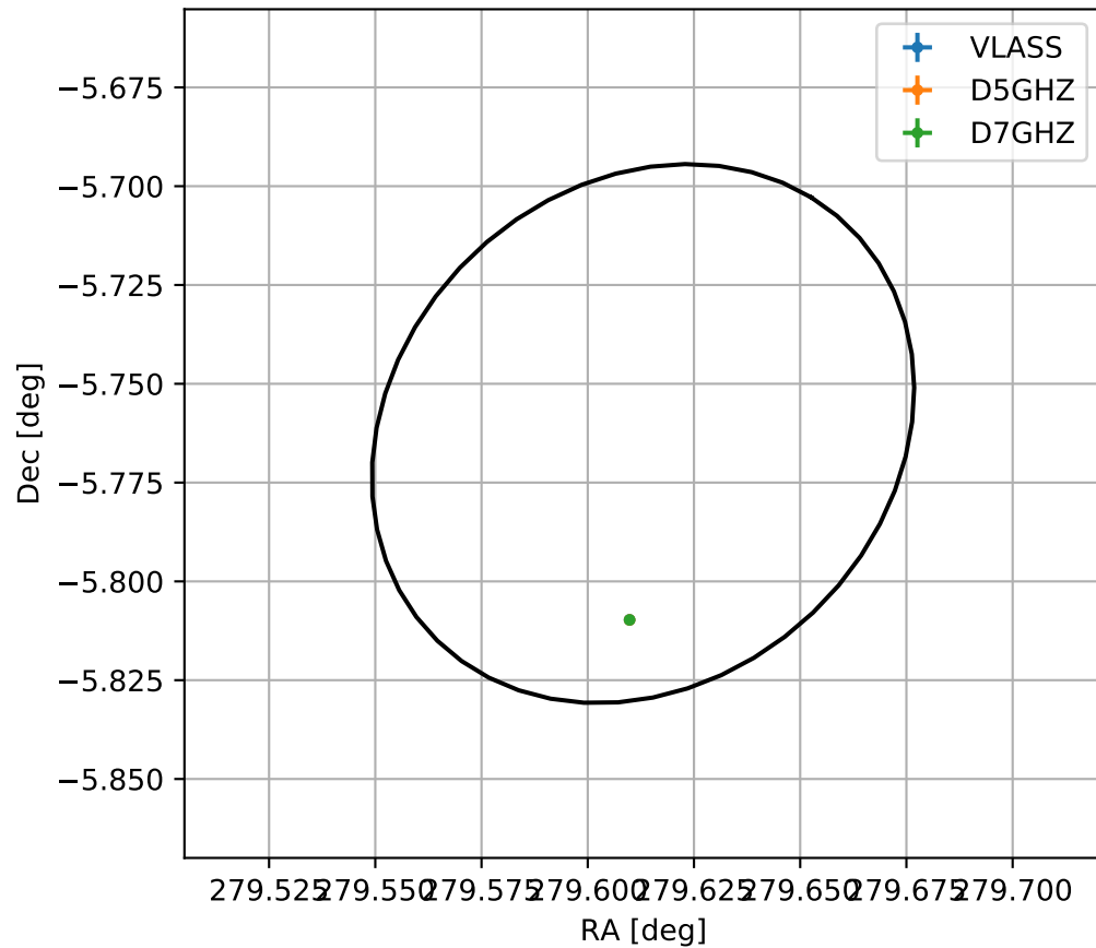
4FGL J1838.4-0545
