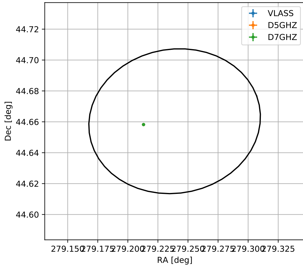
4FGL J1836.9+4439
