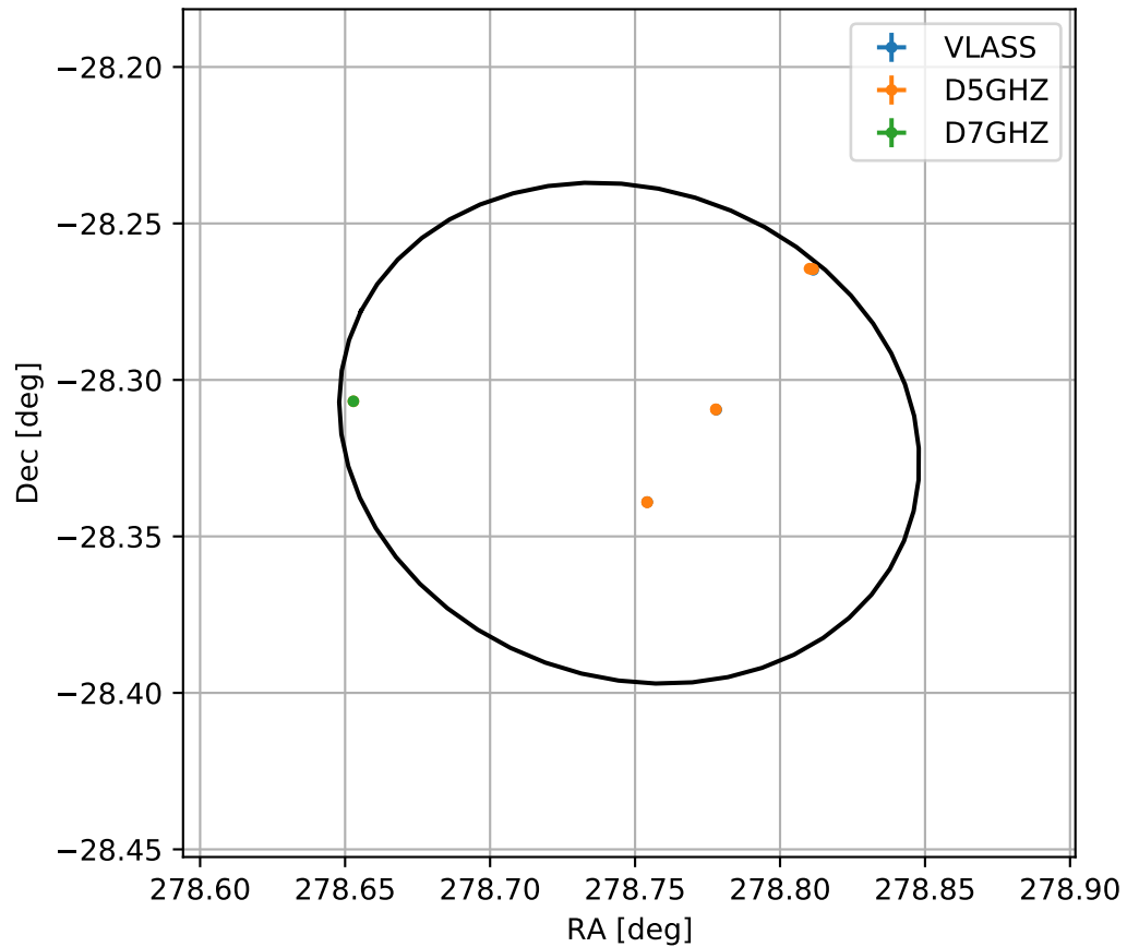
4FGL J1834.9-2819
