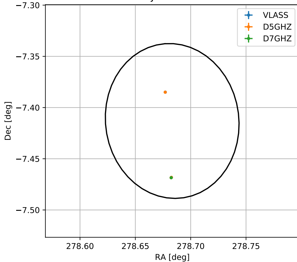
4FGL J1834.7-0724c
