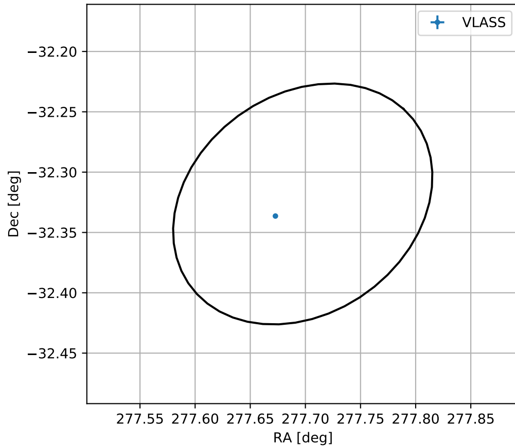
4FGL J1830.7-3219
