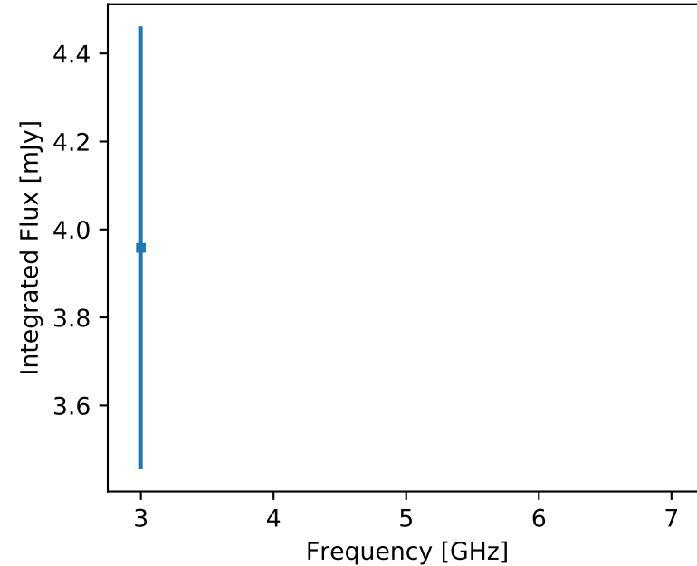
F357 J183041.47-322011.0 (unr)
