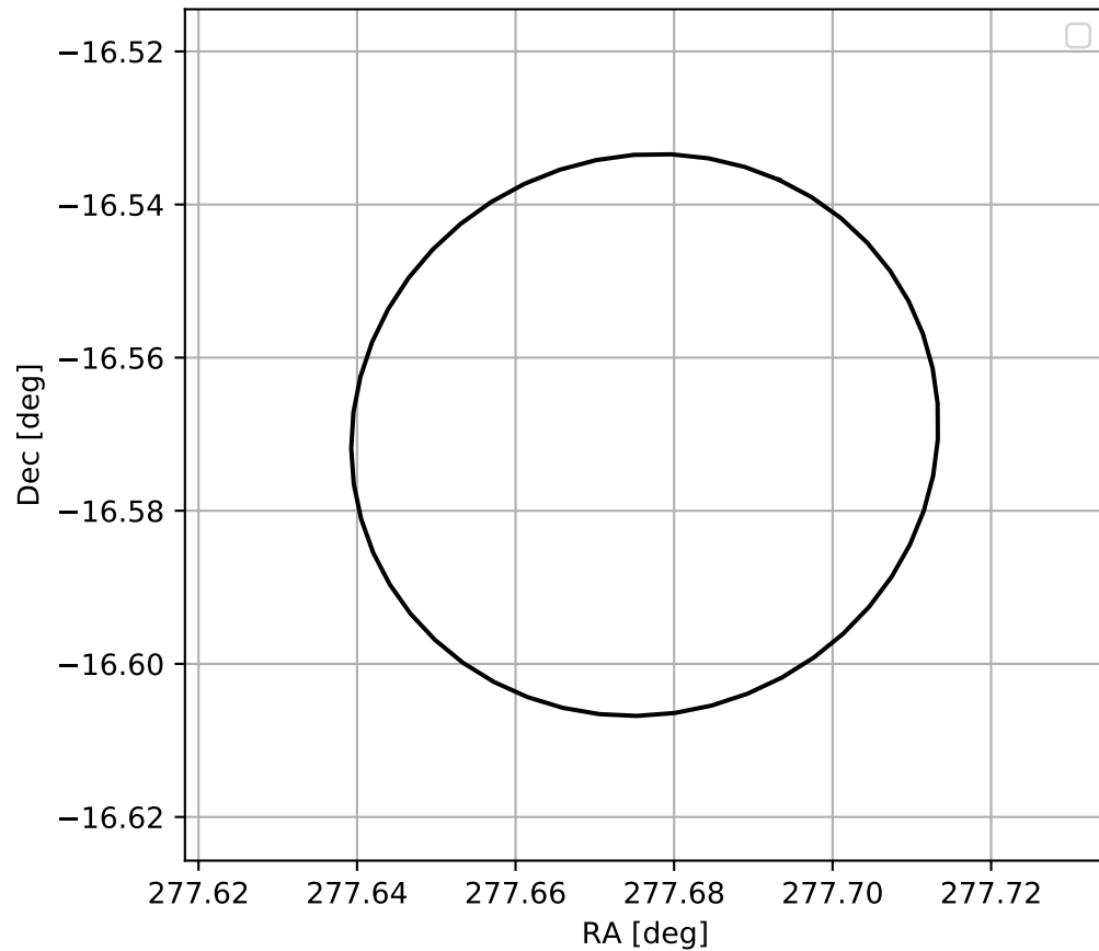
4FGL J1830.7-1634
