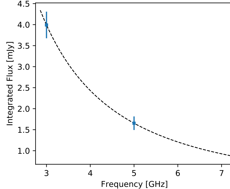
F357 J182954.68-151626.2 (unr)
