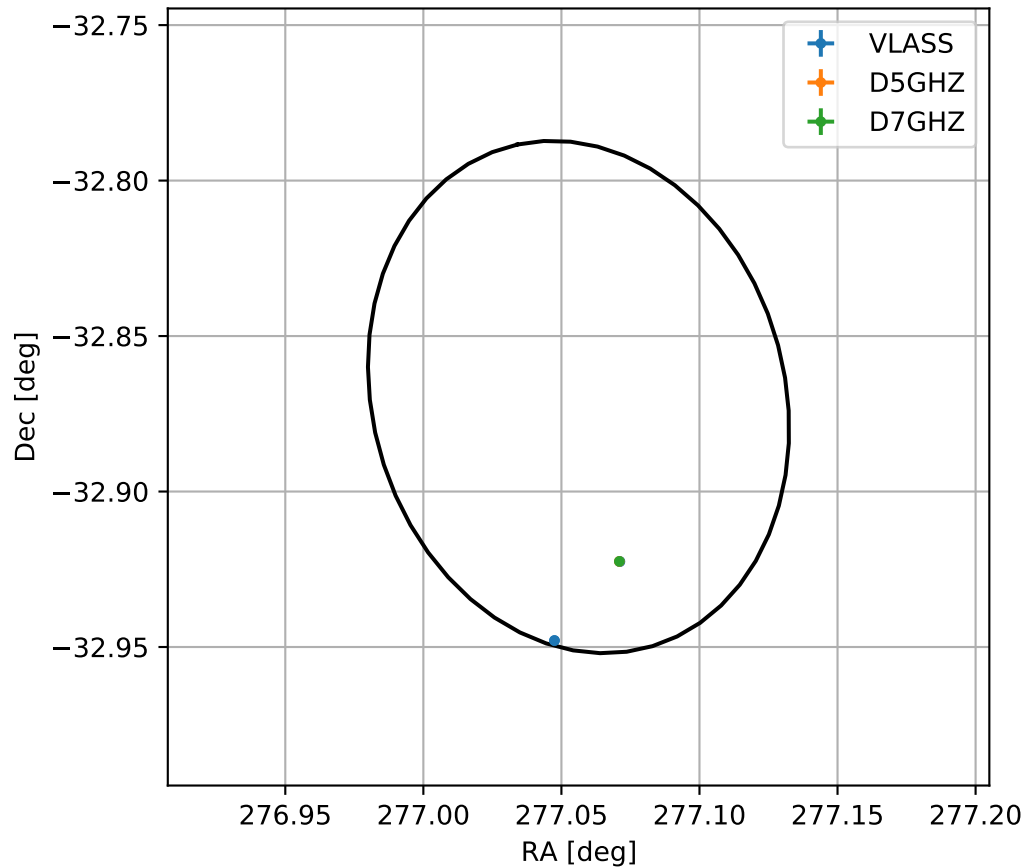
4FGL J1828.2-3252
