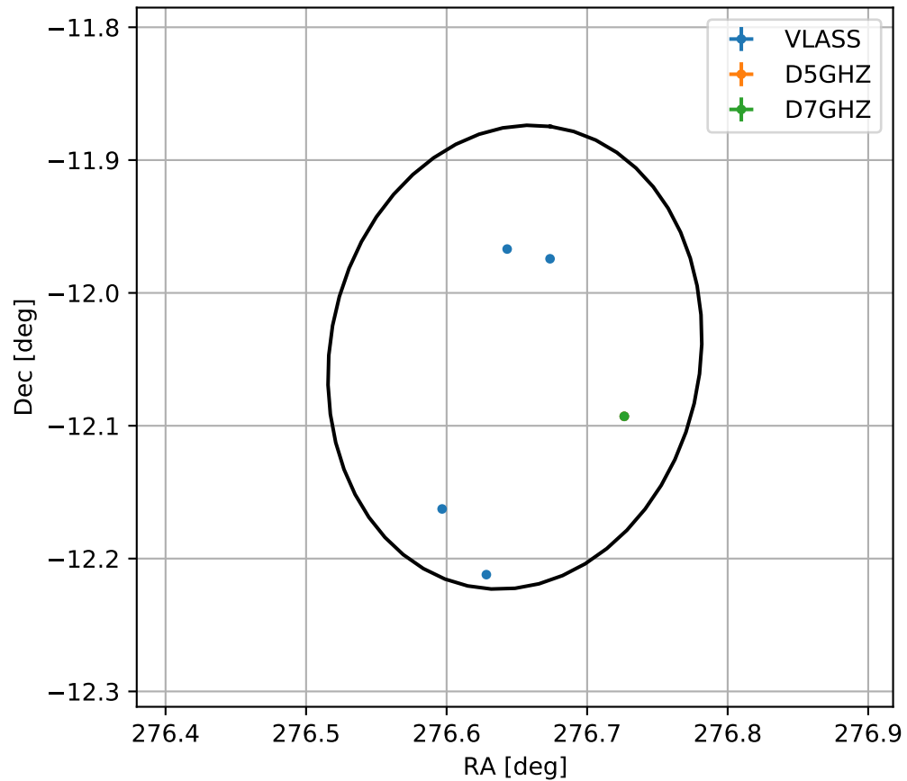
4FGL J1826.5-1202c
