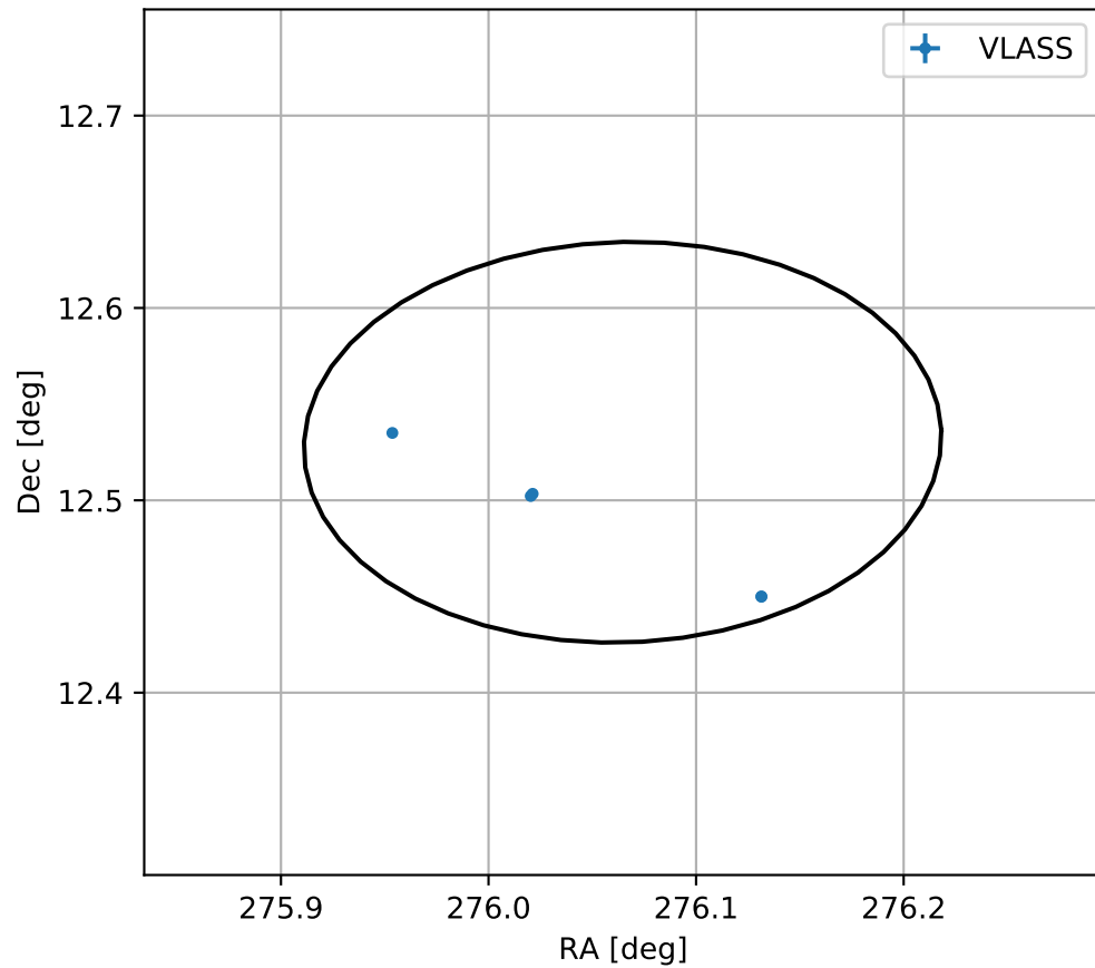
4FGL J1824.2+1231
