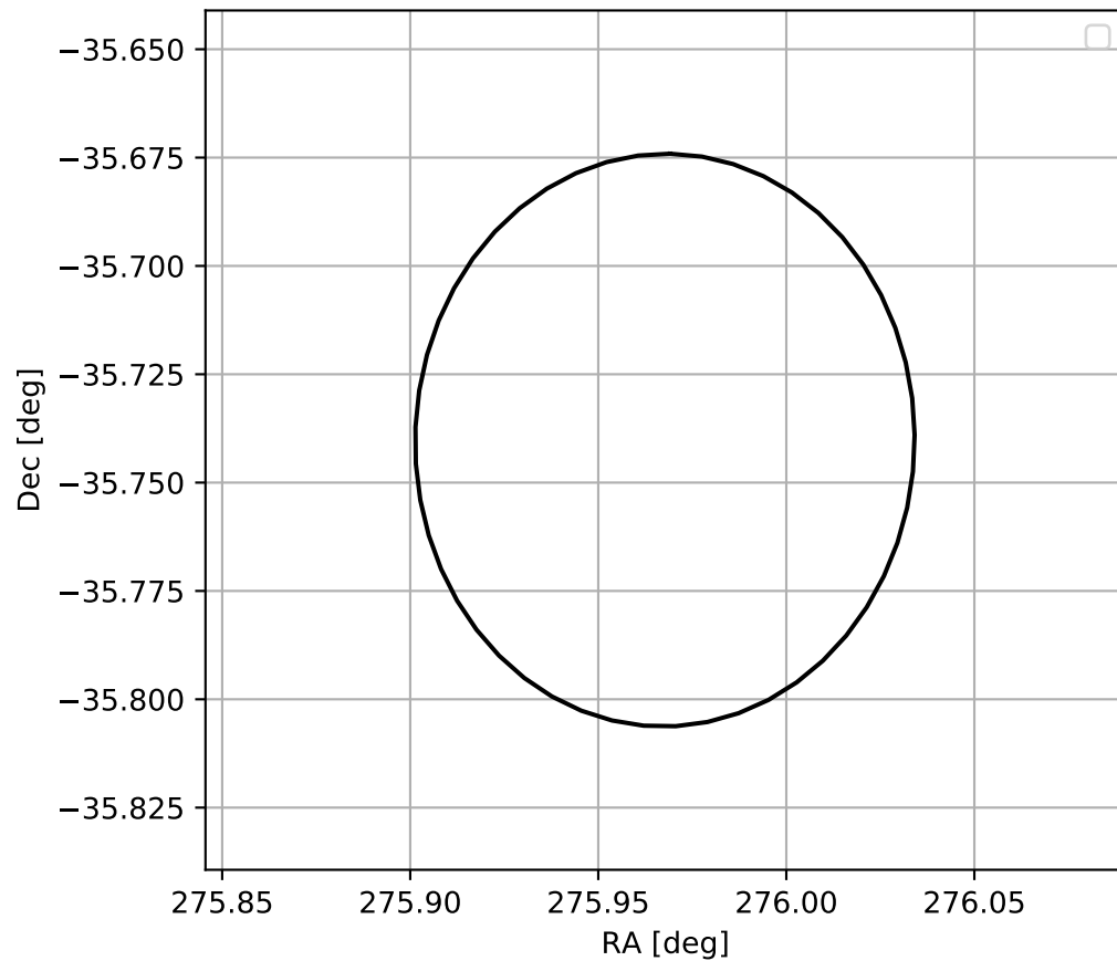
4FGL J1823.8-3544
