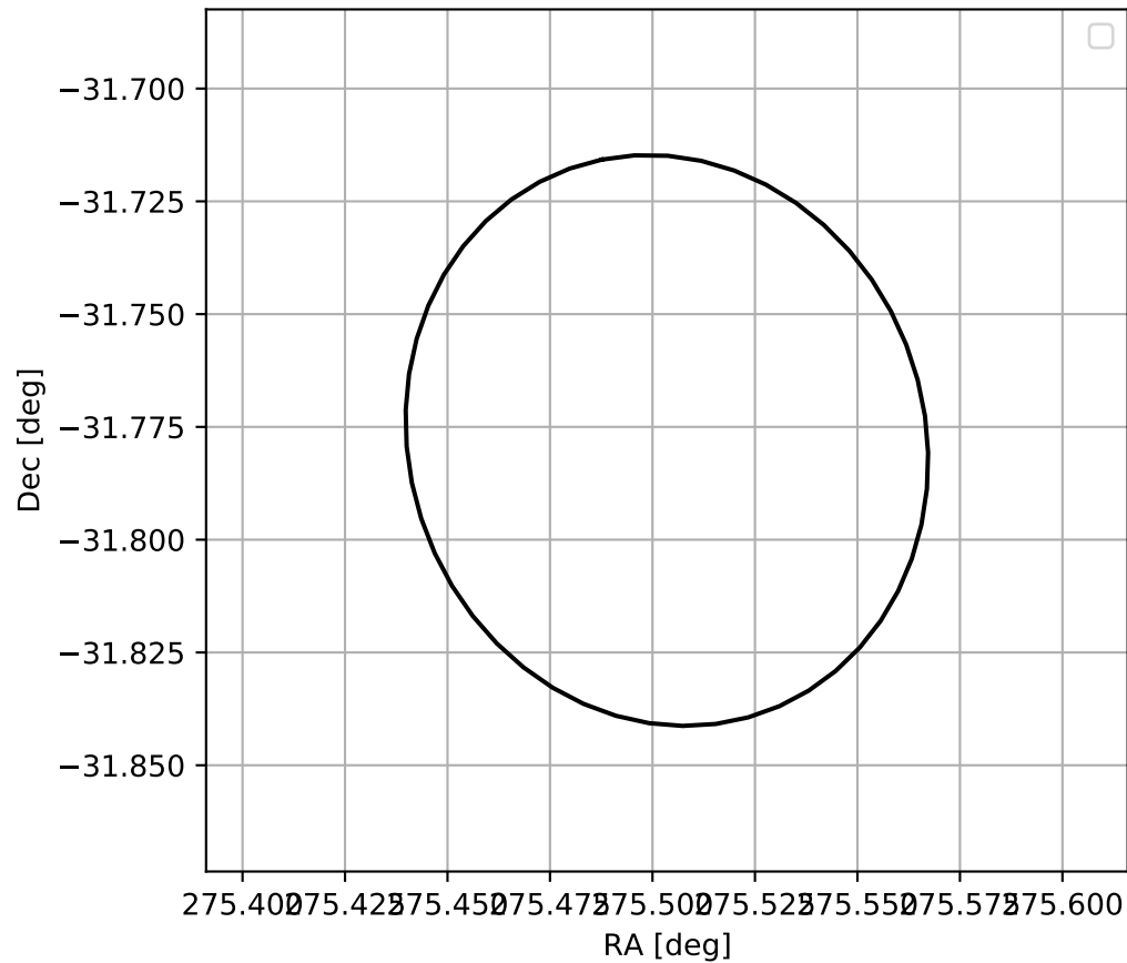
4FGL J1822.0-3146
