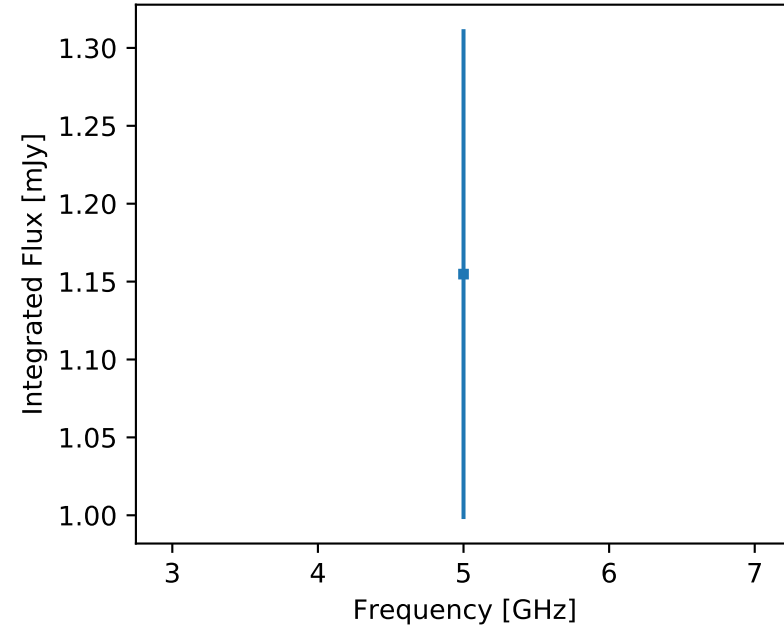
F357 J182140.96-253010.1 (unr)
