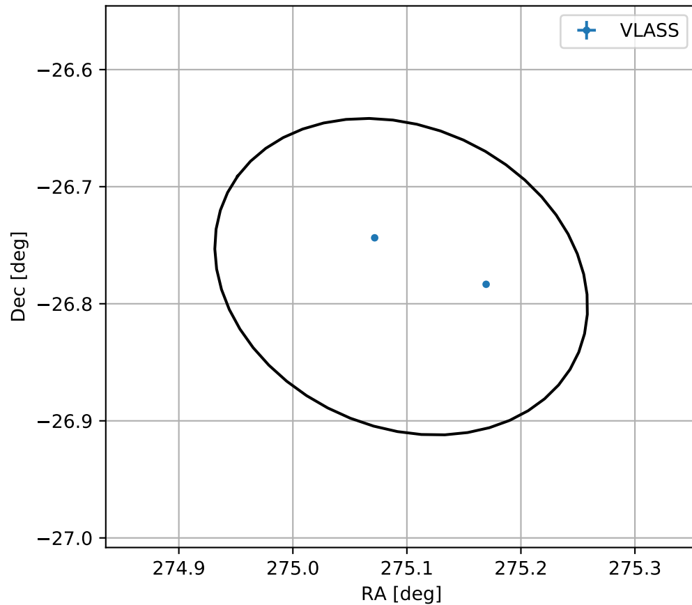
4FGL J1820.3-2646
