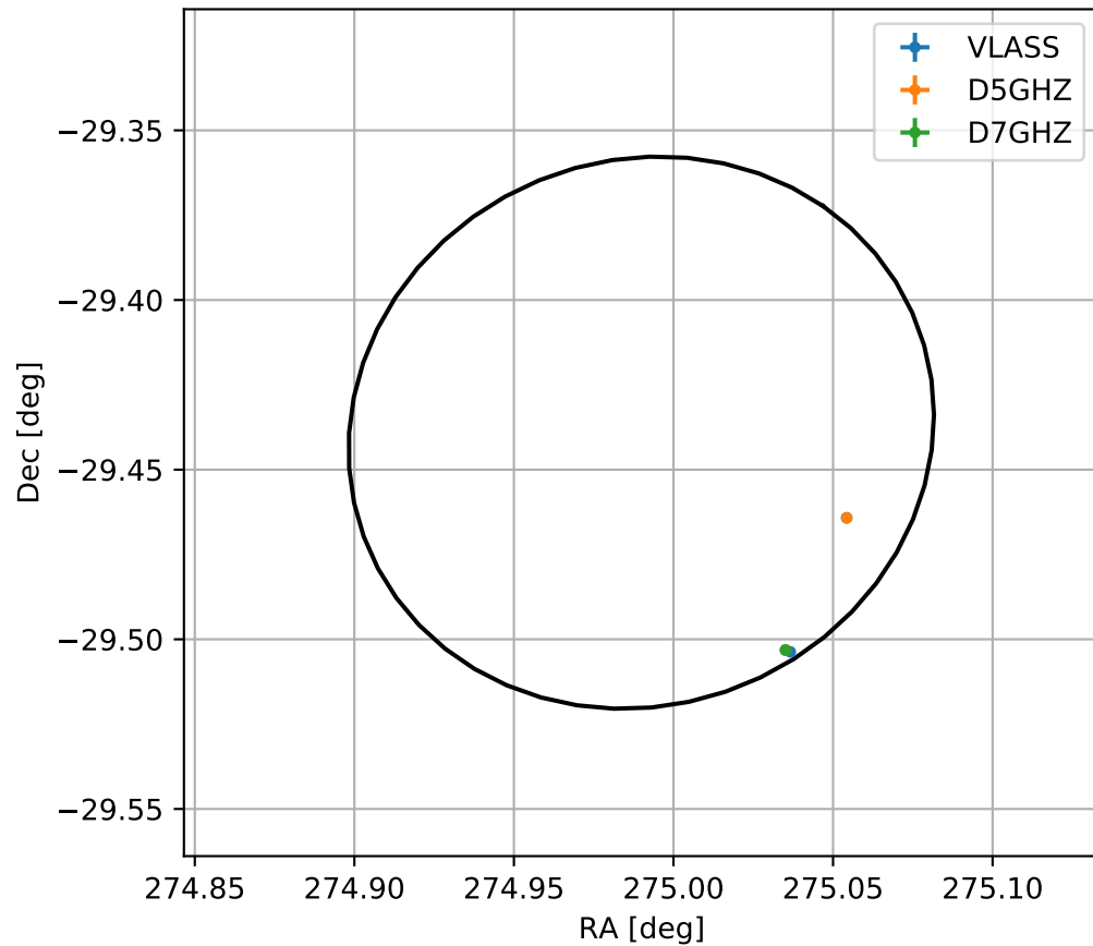
4FGL J1819.9-2926
