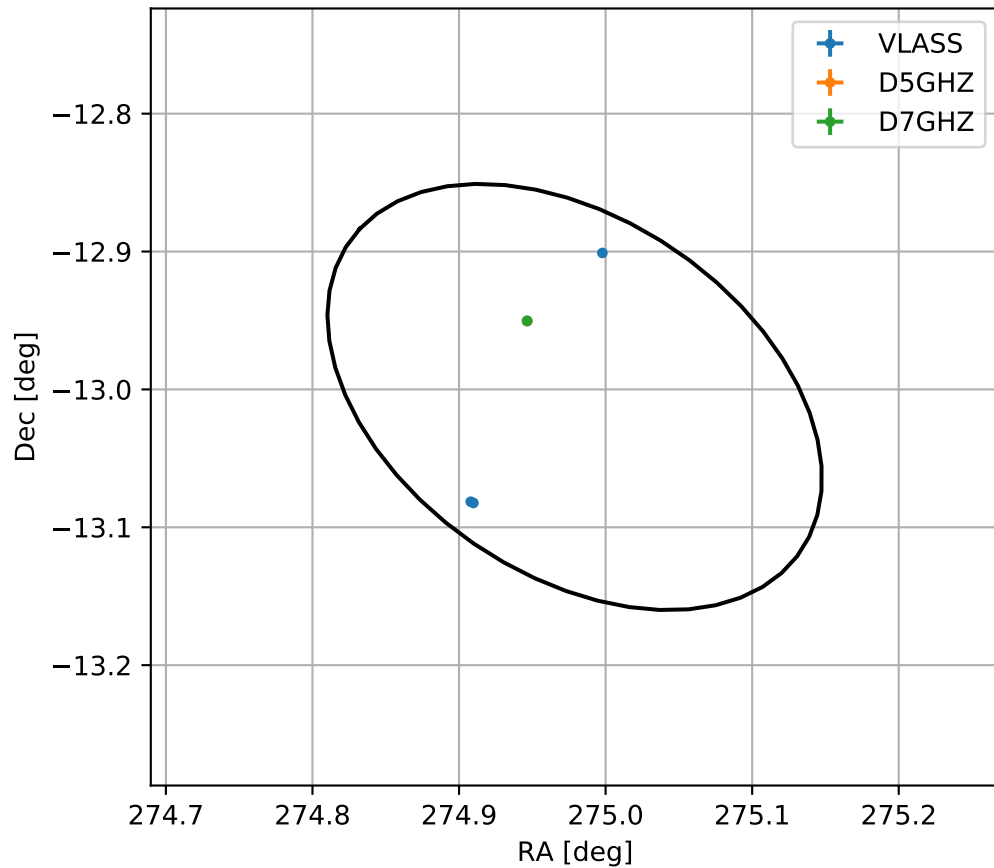
4FGL J1819.9-1300
