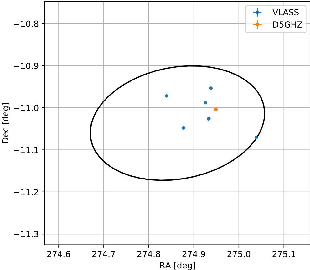
4FGL J1819.4-1102
