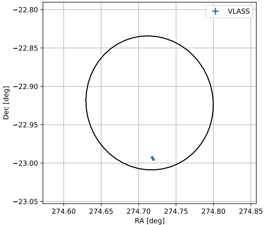
4FGL J1818.8-2255
