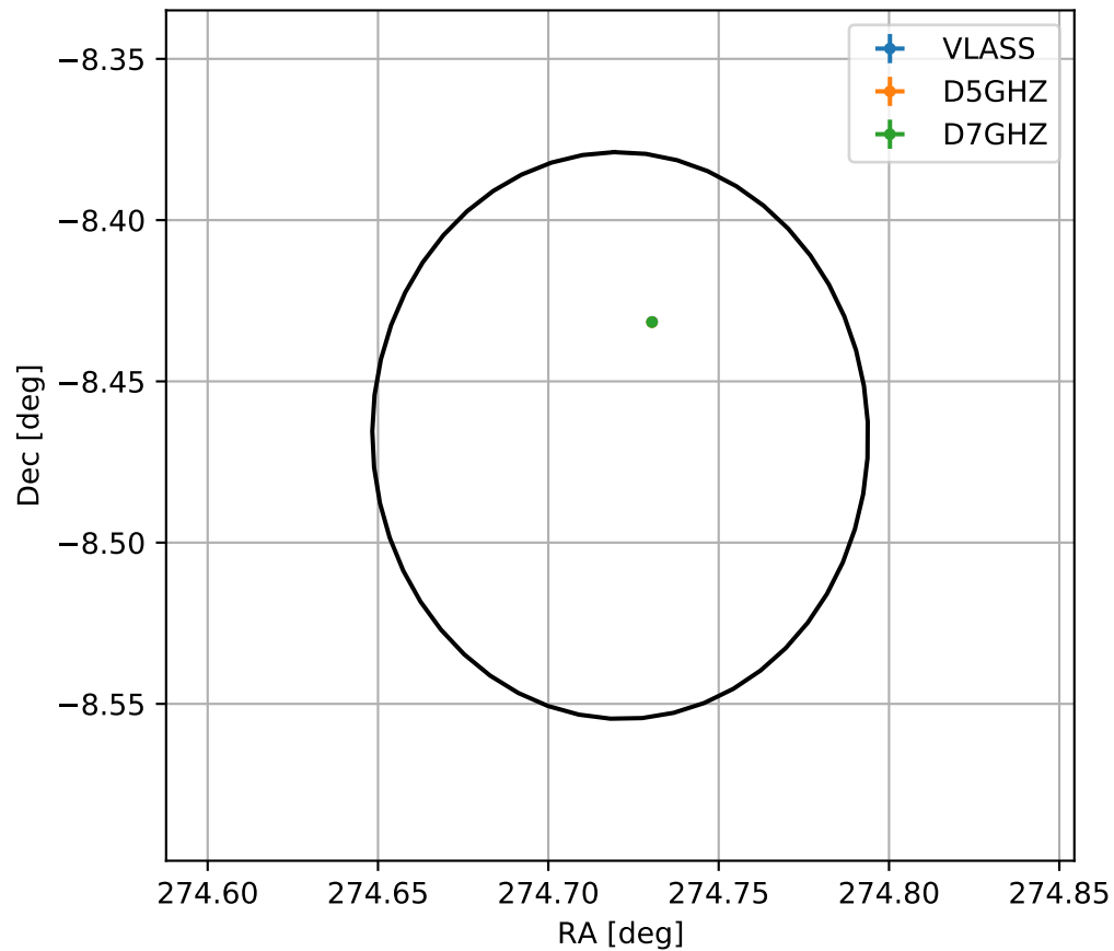
4FGL J1818.8-0828
