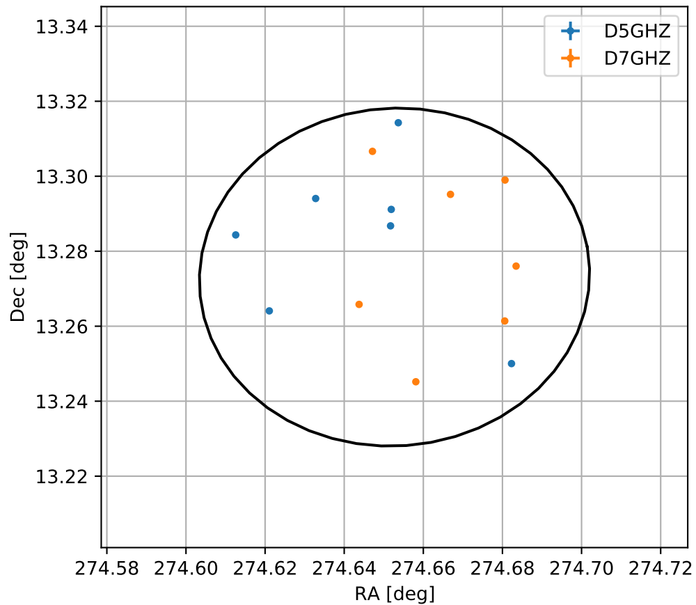
4FGL J1818.6+1316
