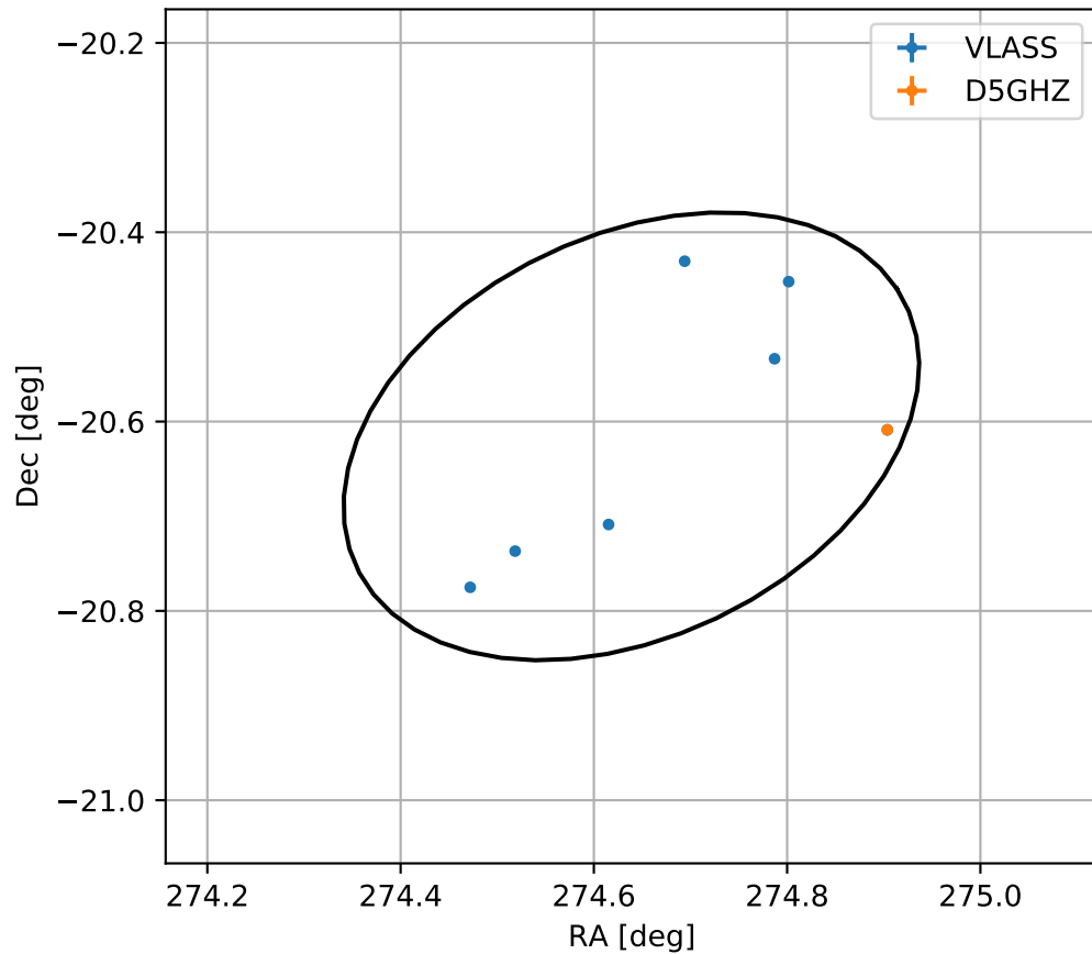
4FGL J1818.5-2036
