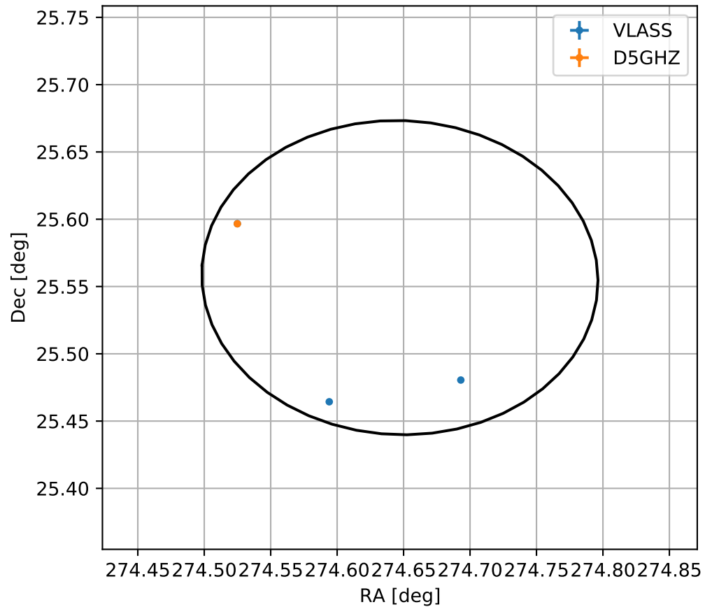
4FGL J1818.5+2533
