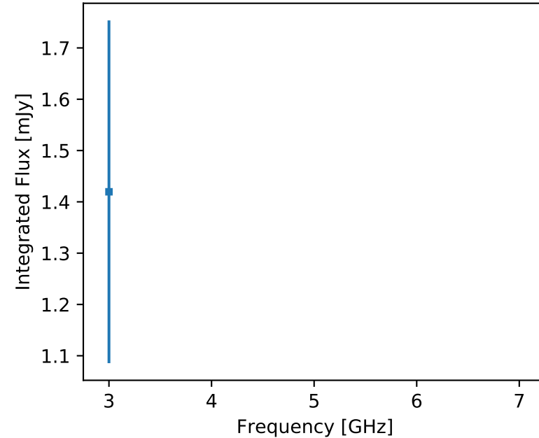
F357 J181802.26-123223.9 (unr)
