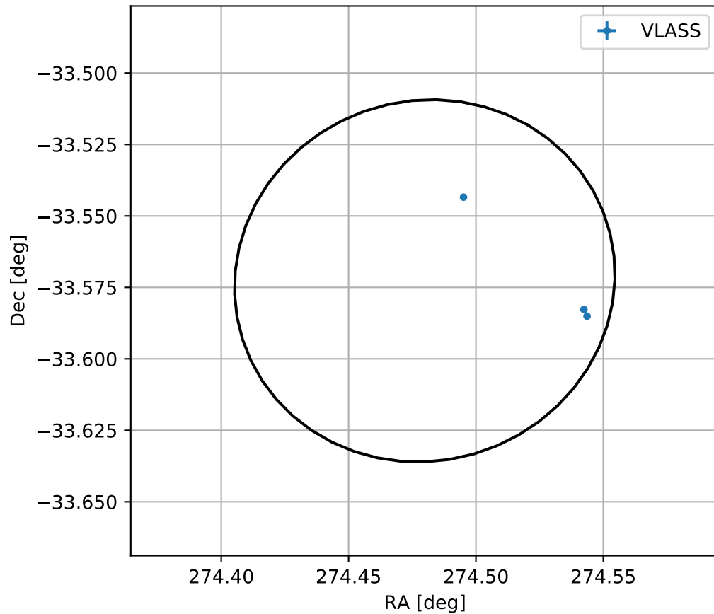
4FGL J1817.9-3334
